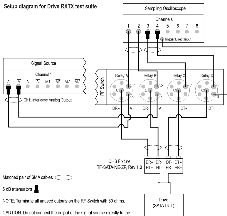
Setup diagram for Drive RXTX test suite
